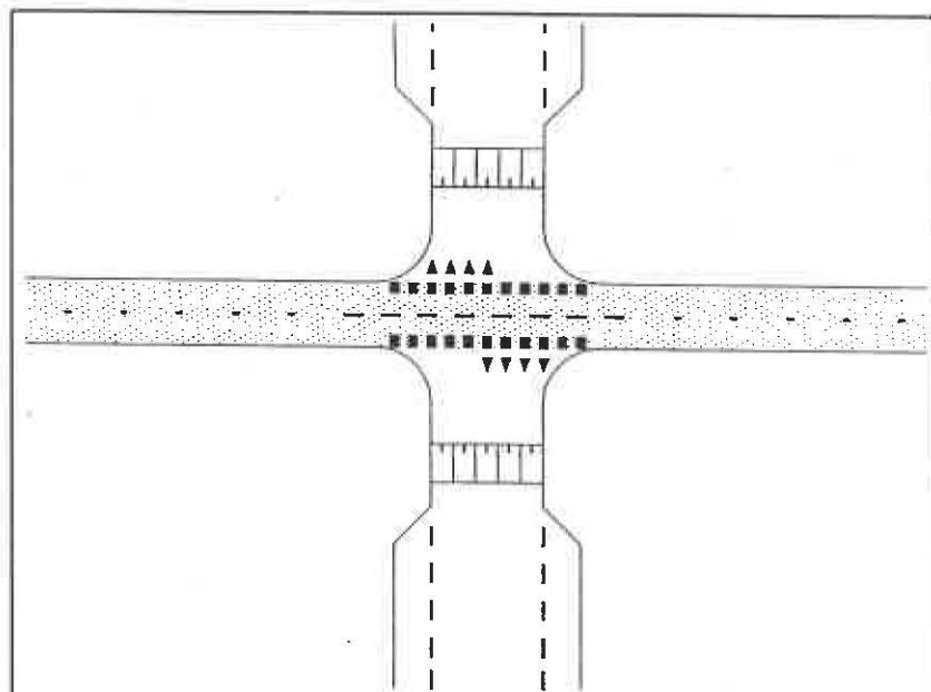
Fig 6: Cycle route with Right of Way over crossing road
