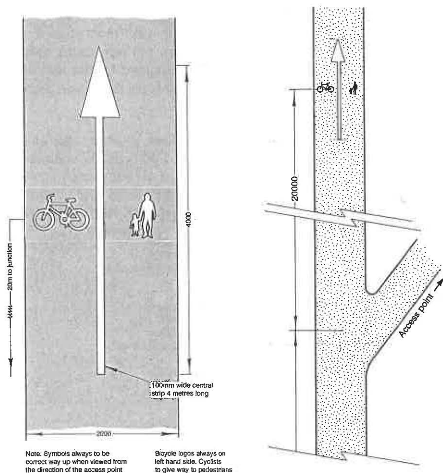
Fig 19: Shared use path markings
