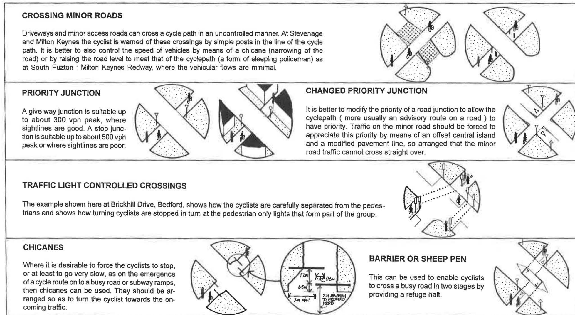
Fig 1: Highway Crossings - Traffic engineering solutions. Sometimes the highway will have to be crossed at grade. Here are some options.
